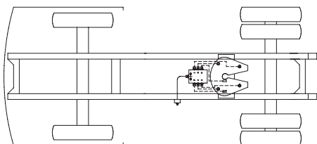
Practical example, fifth-wheel support plate: usually 6 lube points
