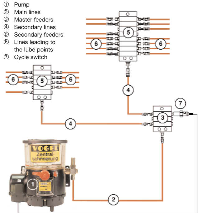
Diagram of a progressive centralized lubrication system
